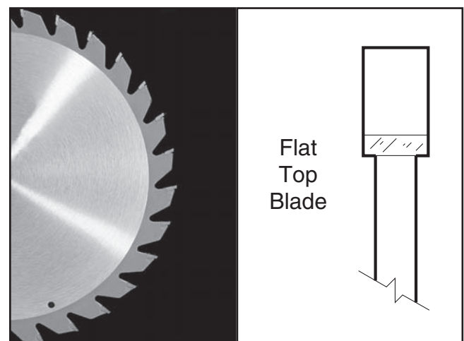
Figure 44. Ripping blade.
